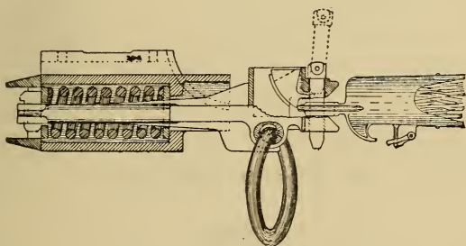
FIG. 41.—THE SPRING DRAW BAR.
